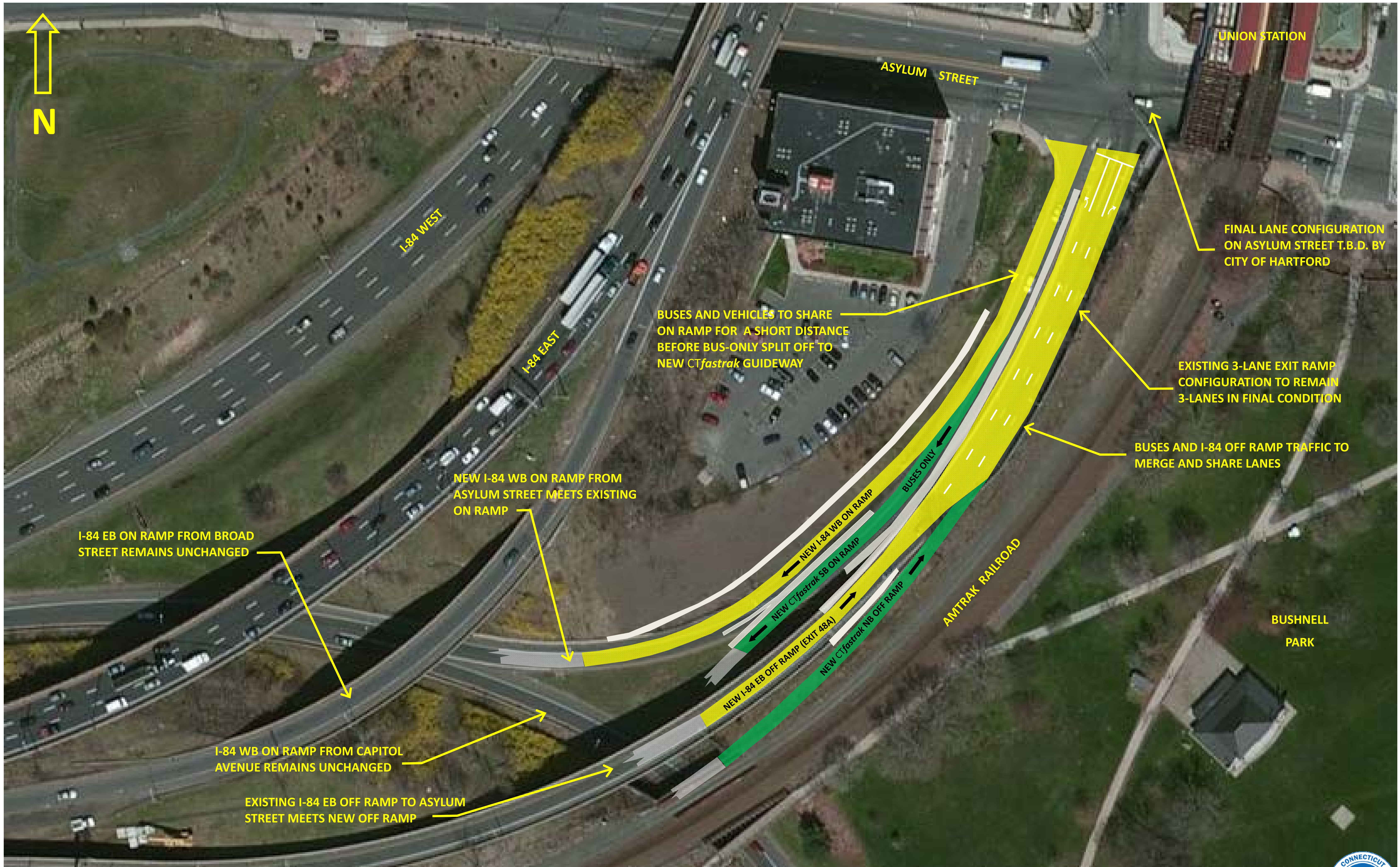
NEW GUIDEWAY AND I-84 EXIT/ENTRY RAMPS AT ASYLUM STREET IN HARTFORD FINAL CONFIGURATION
